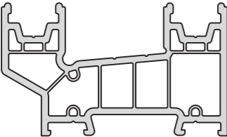
LPD081 Outer Frame
